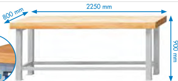
MOD. 200 VS
