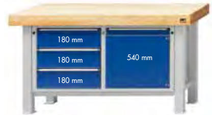
MOD. 106 VS
