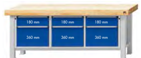
MOD. 223 VS
